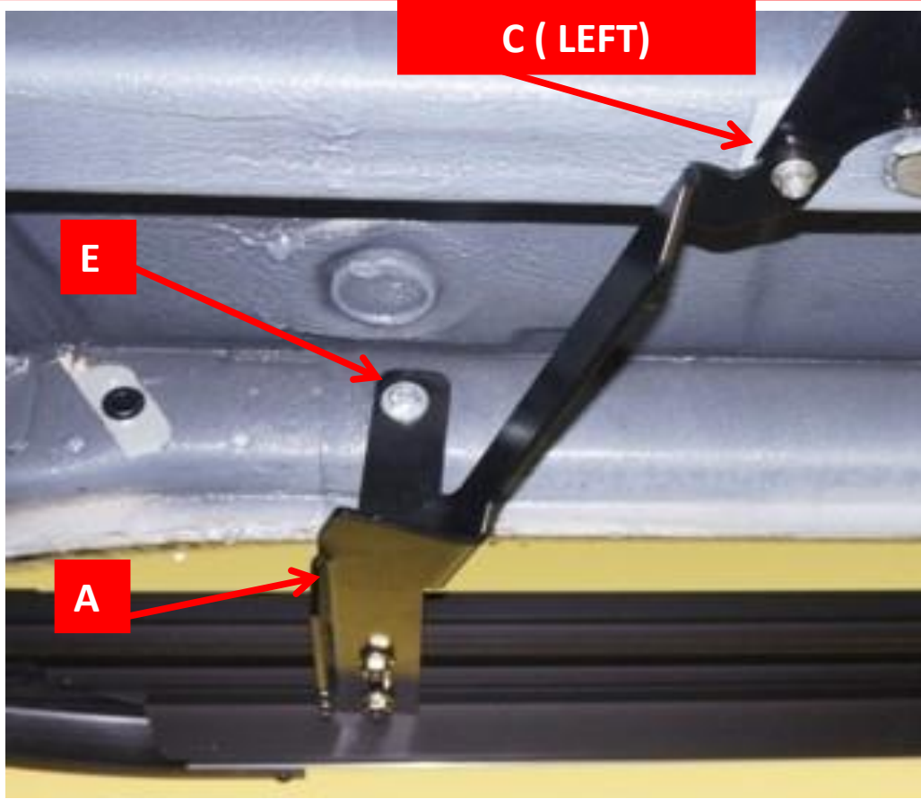
FRONT BRACKET
