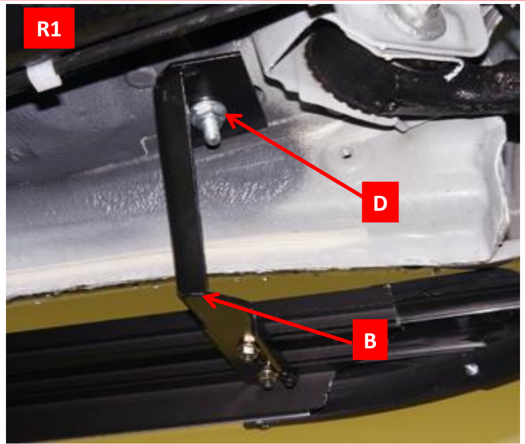
REAR BRACKET
