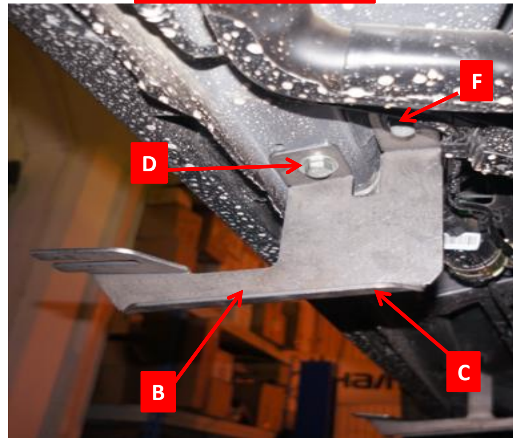
REAR BRACKET
