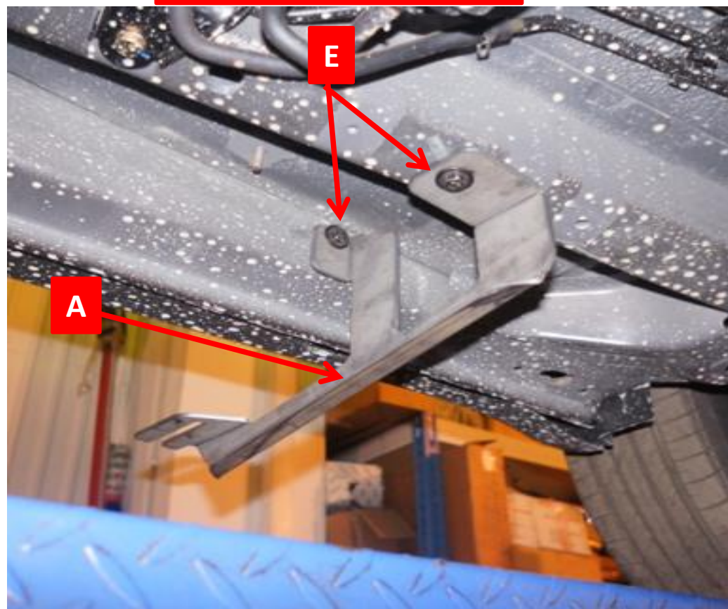
FRONT BRACKET
